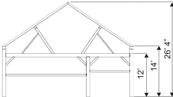
BENT VIEW
